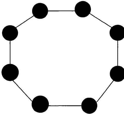
One-dimensional cellular space: finite ring (circular boundary conditions)
