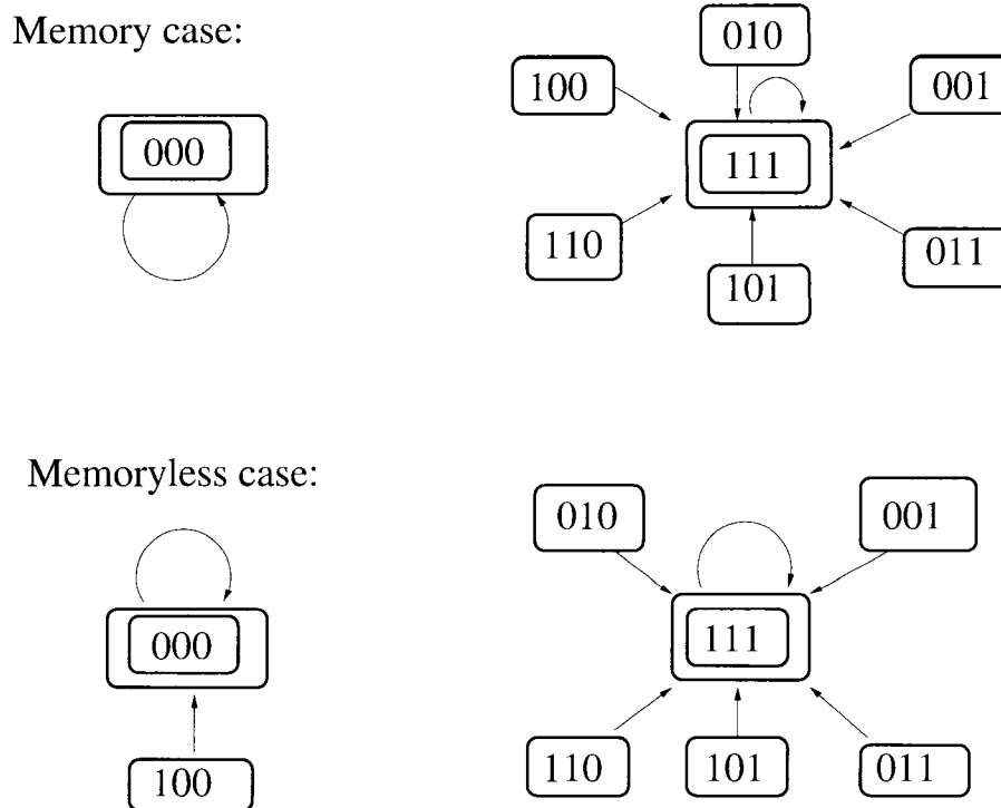
Figure 5.2: Configuration space of the Boolean SDS given in Figure 5.1.
