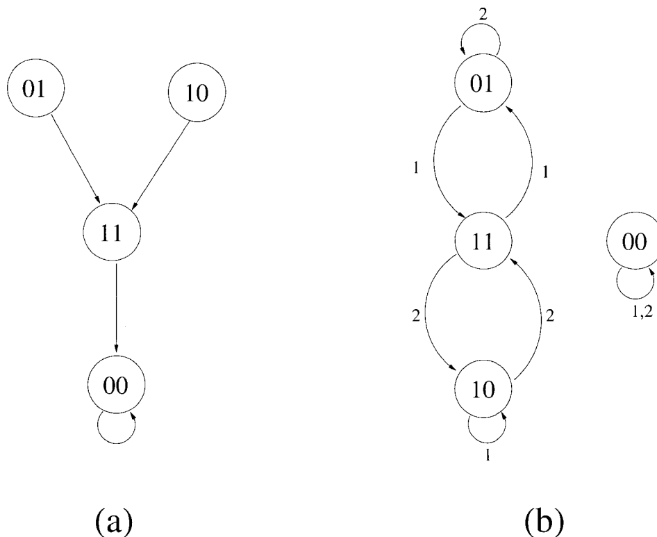
Figure 4.2: Configuration spaces for the two-node (a) parallel and (b) sequential cellular automata with \delta = XOR , respectively
