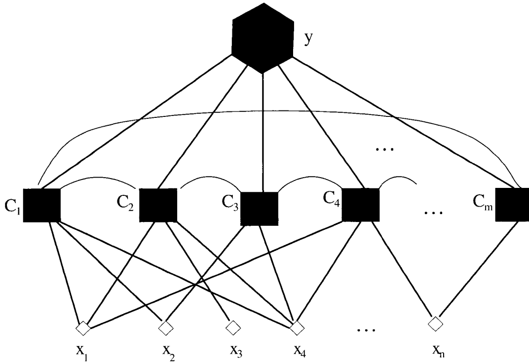
Figure 5.3: The graph of a symmetric Boolean SyDS in the construction of Theorem 5.6.
