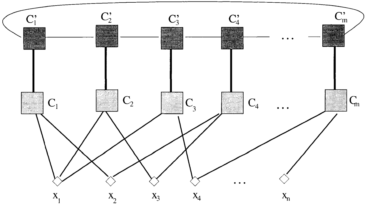
Figure 6.1: The underlying graph of a bounded-degree monotone linear threshold Boolean S(y) DS in the construction of Theorem 6.3.
