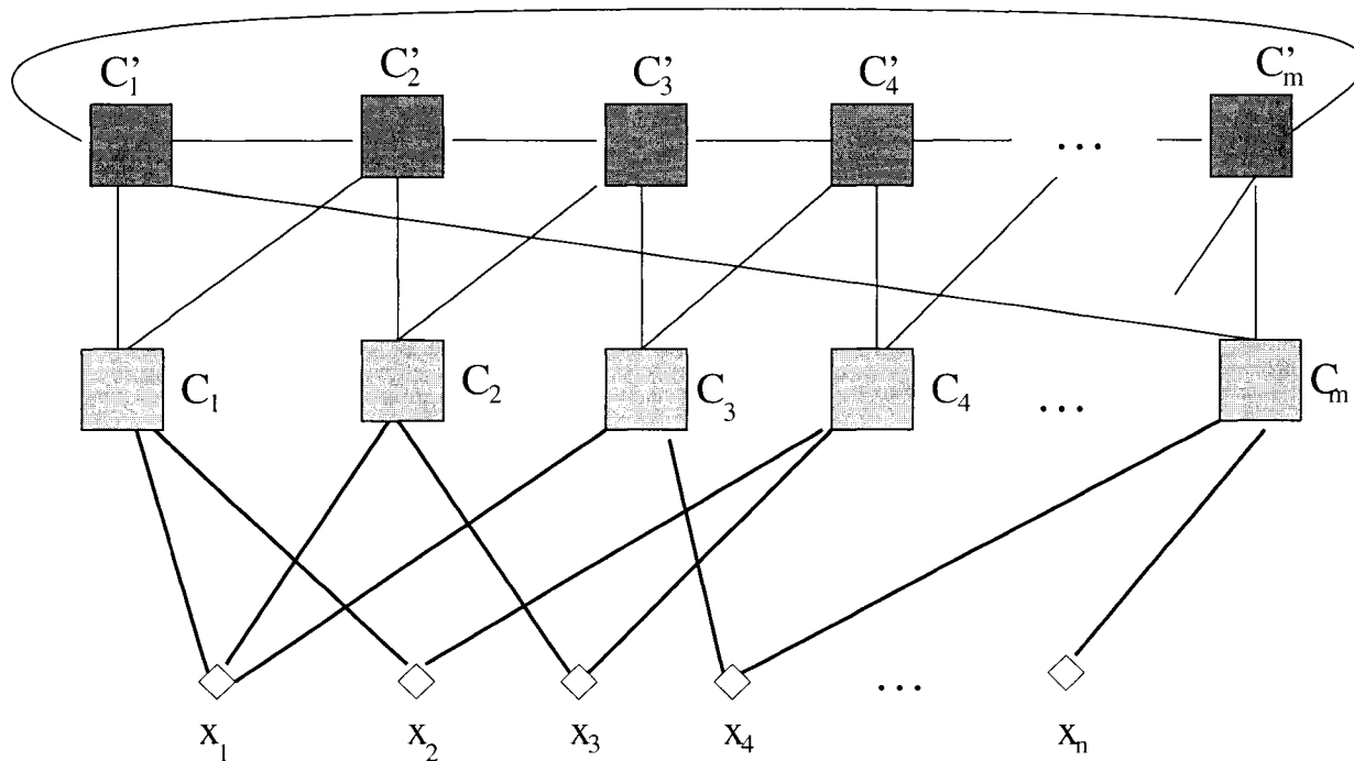
Figure 6.2: The underlying graph of a bounded-degree simple threshold Boolean S(y)DS in the construction of Theorem 6.6.
