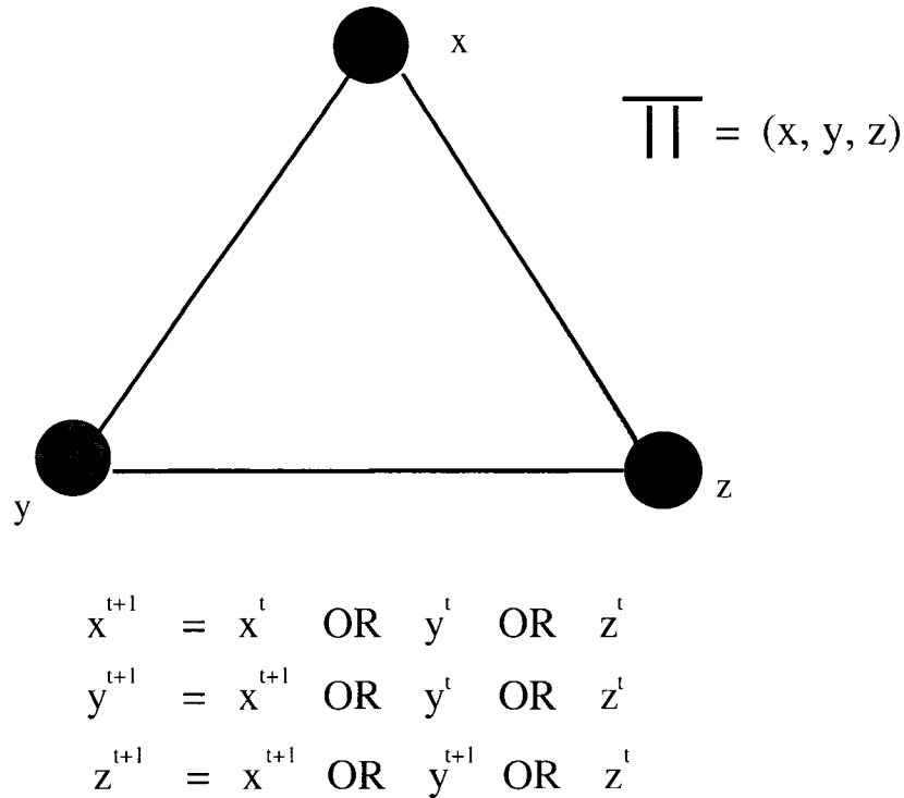
Figure 5.1: A Boolean SDS with three interconnected nodes. Each node locally updates its state according to the Boolean OR function. The sequence of node updates is \Pi^\omega = (x, y, z)^\omega .
